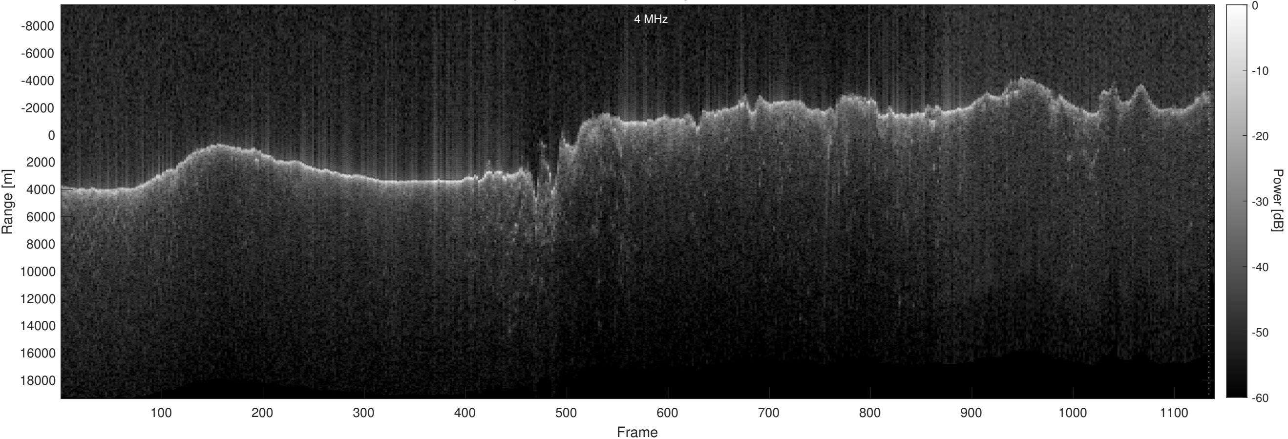
Orbit 13378, Optimized, No Window, Depth-Corrected, Channel 2
