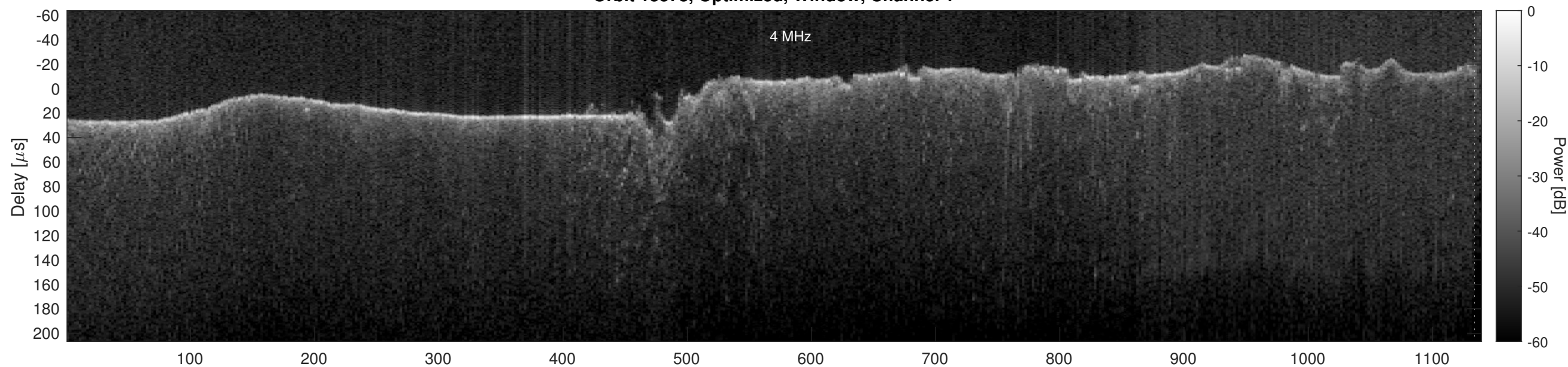
Orbit 13378, Optimized, Window, Channel 2
