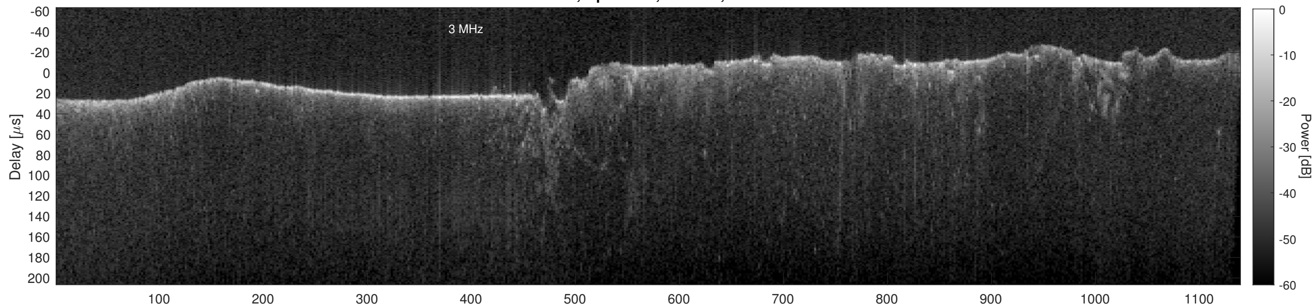
Orbit 13378, Cluttergram
