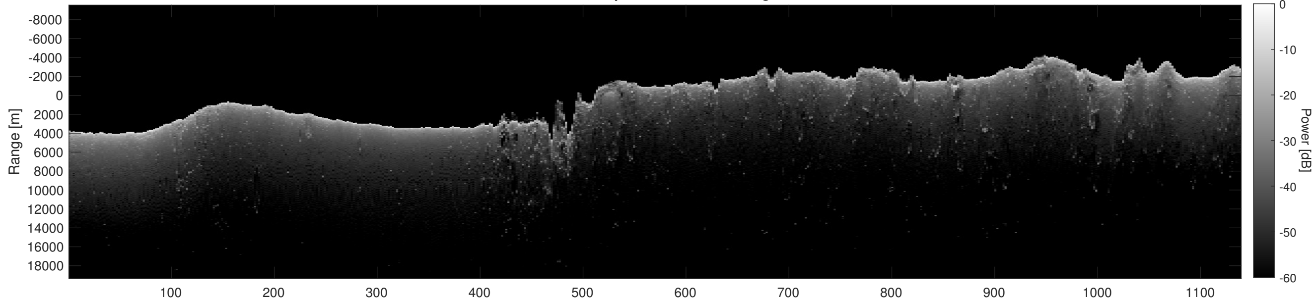
Orbit 13378, Depth-Corrected Cluttergram
