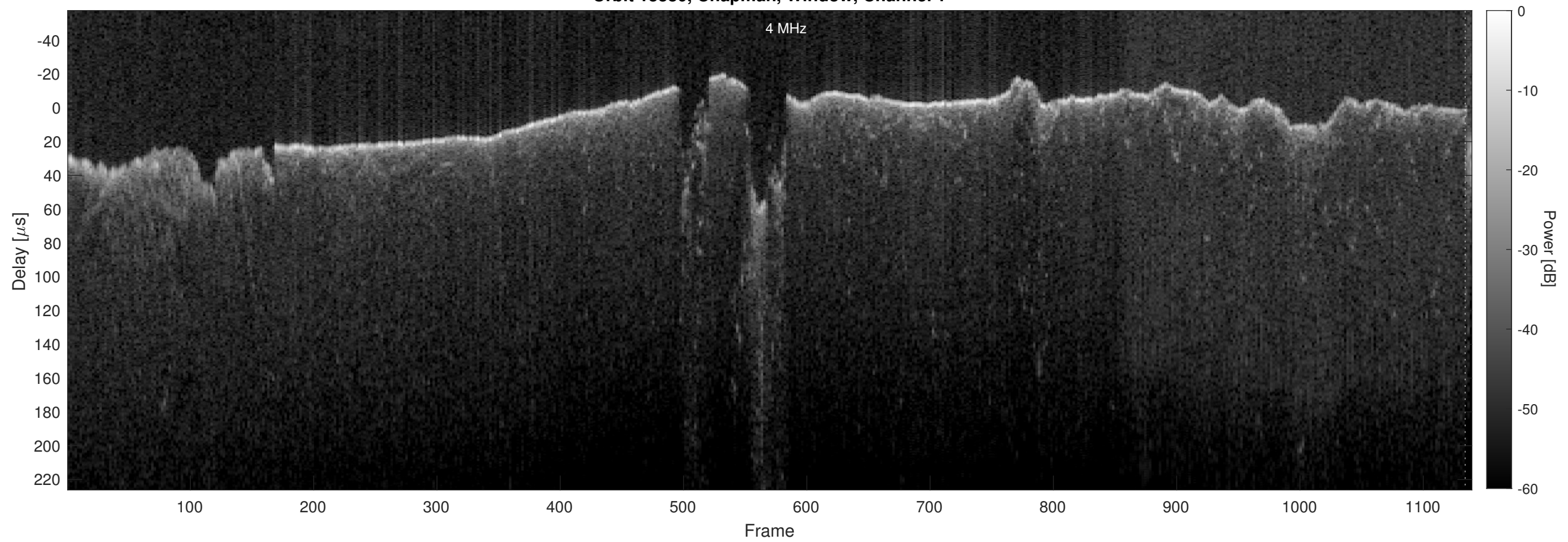
Orbit 13380, Chapman, Window, Channel 2
