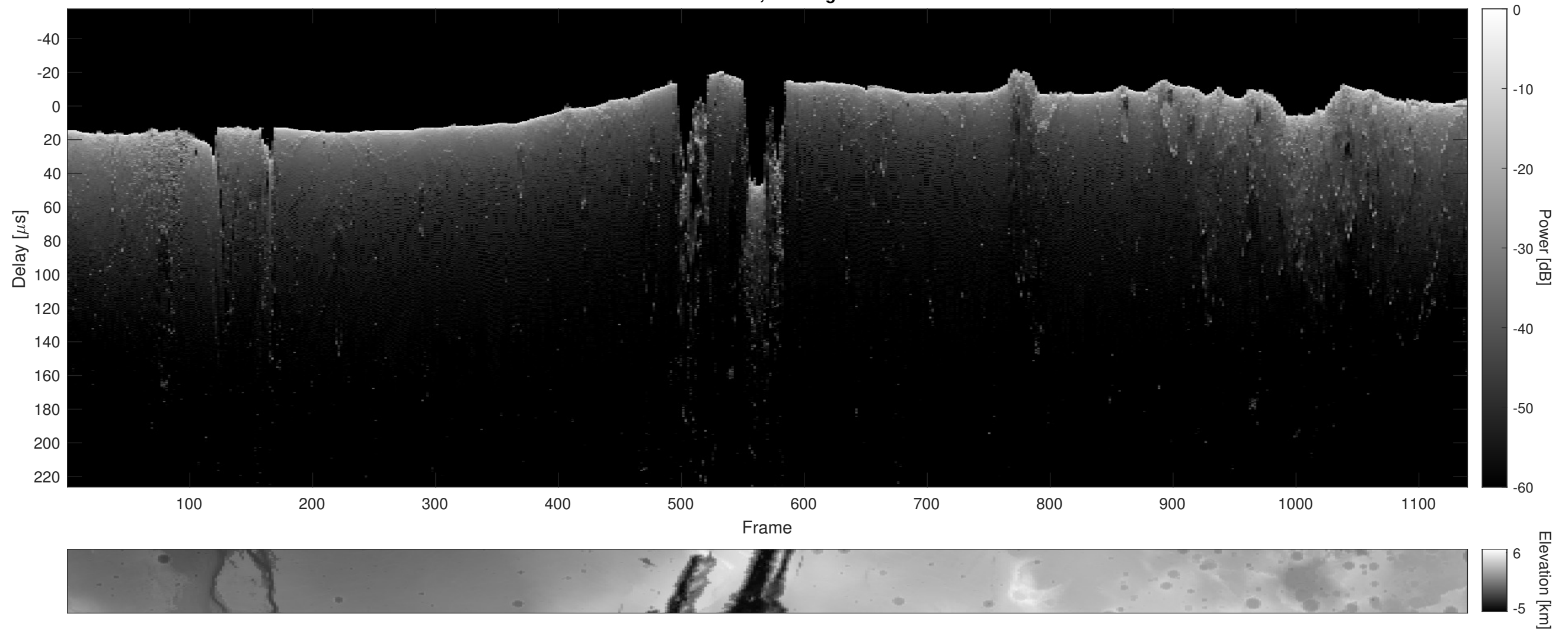
Orbit 13380, Cluttergram
