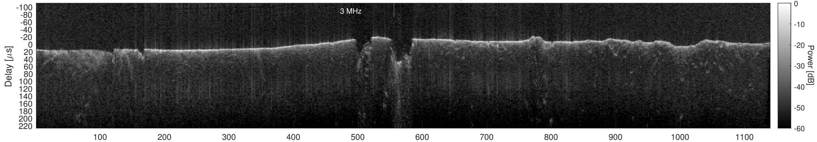
Orbit 13380, Cluttergram
