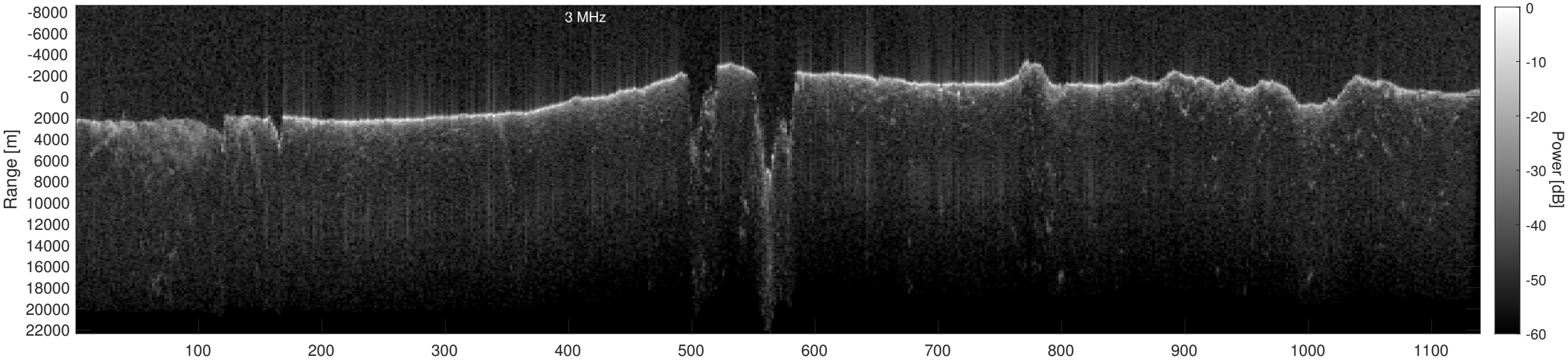
Orbit 13380, Depth-Corrected Cluttergram
