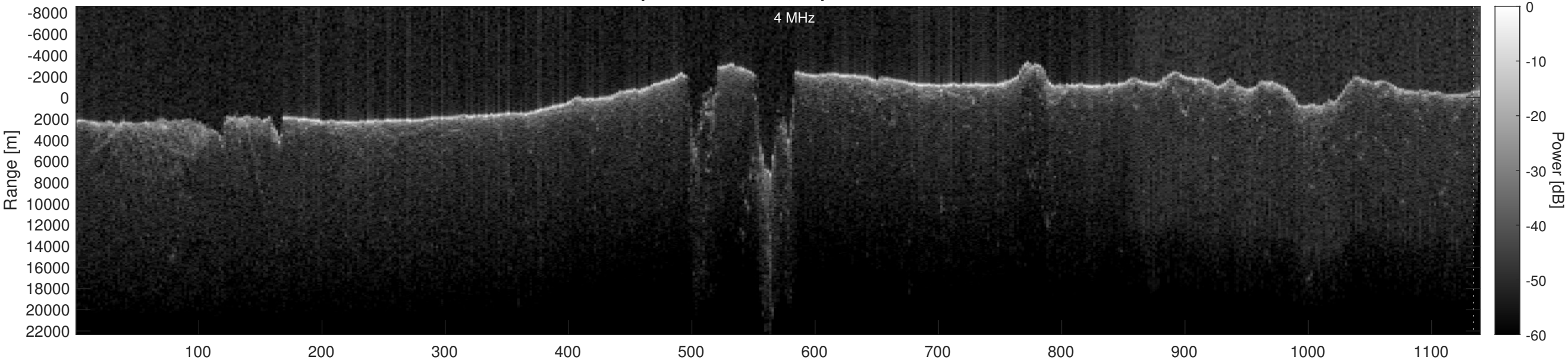
Orbit 13380, Optimized, Window, Depth-Corrected, Channel 2
