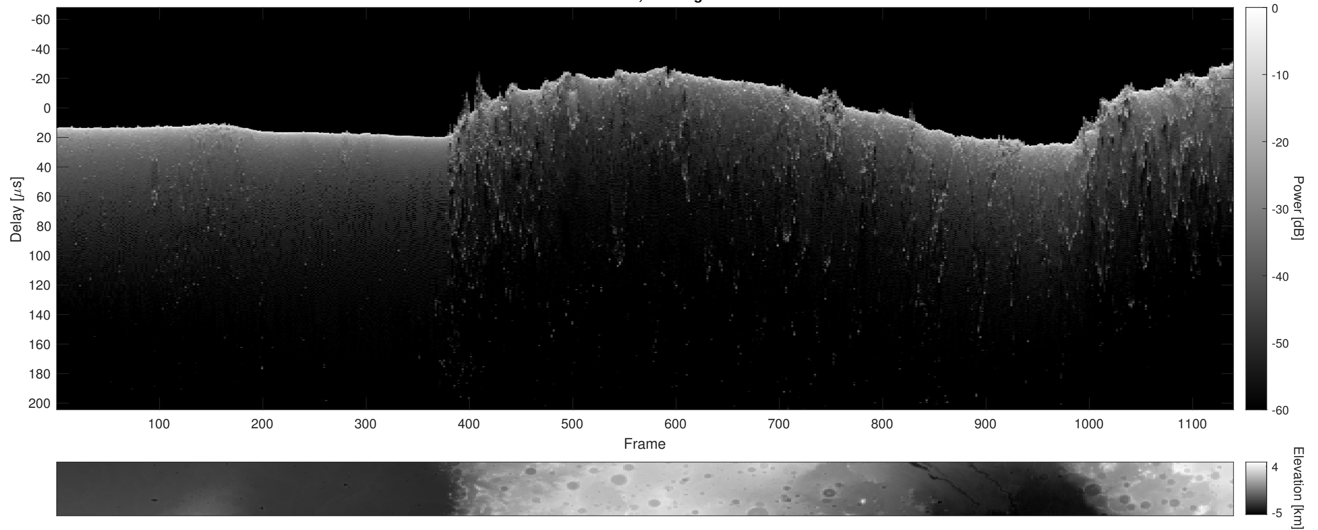
Orbit 13382, Cluttergram
