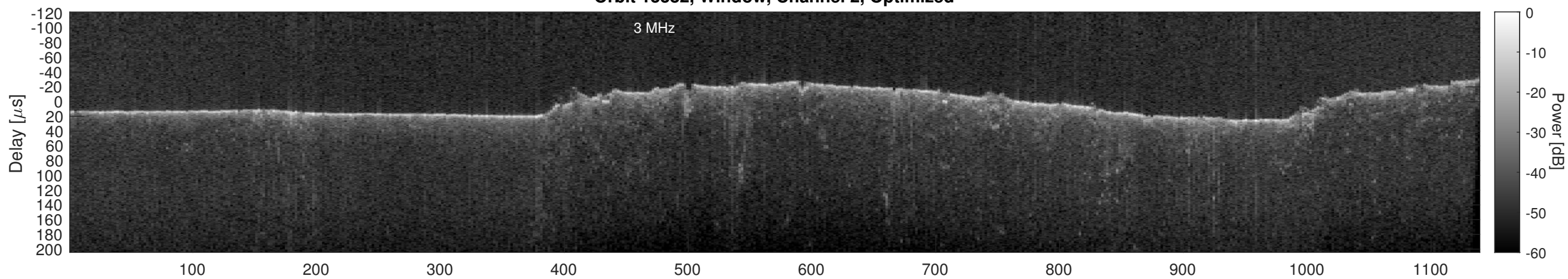
Orbit 13382, Cluttergram
