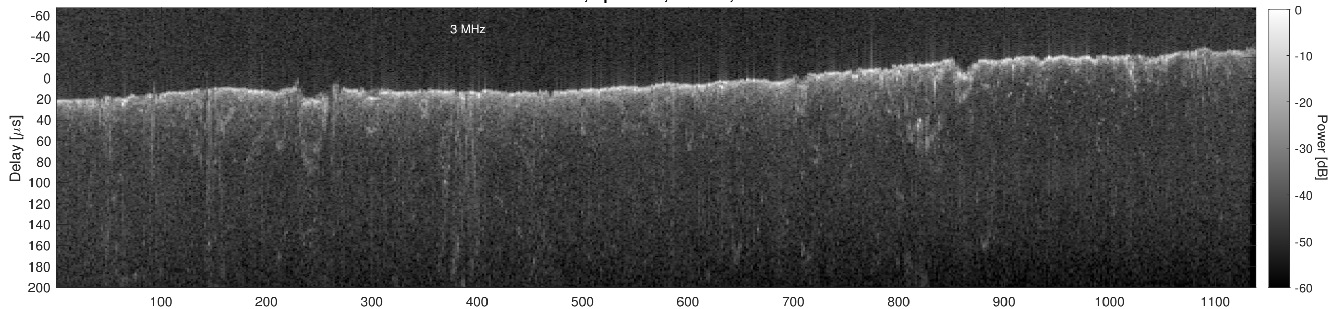
Orbit 13383, Cluttergram
