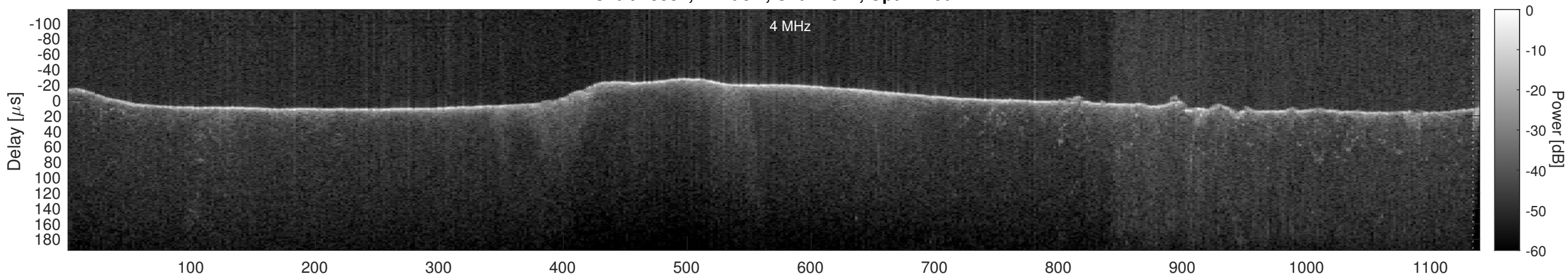
Orbit 13384, Cluttergram
