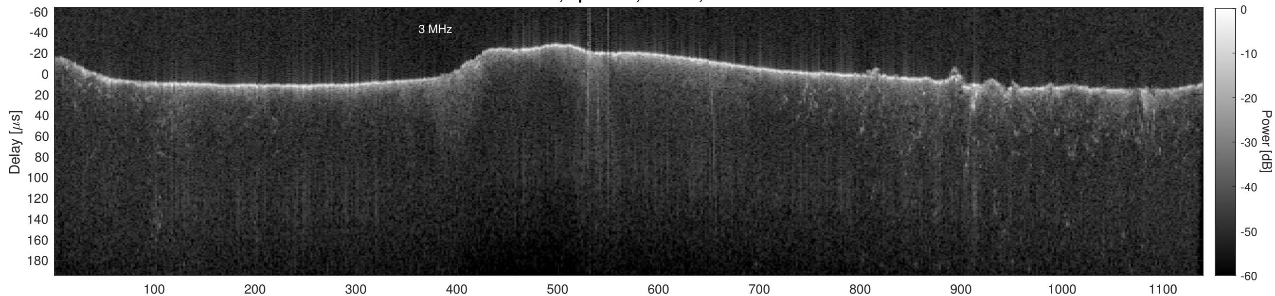
Orbit 13384, Cluttergram
