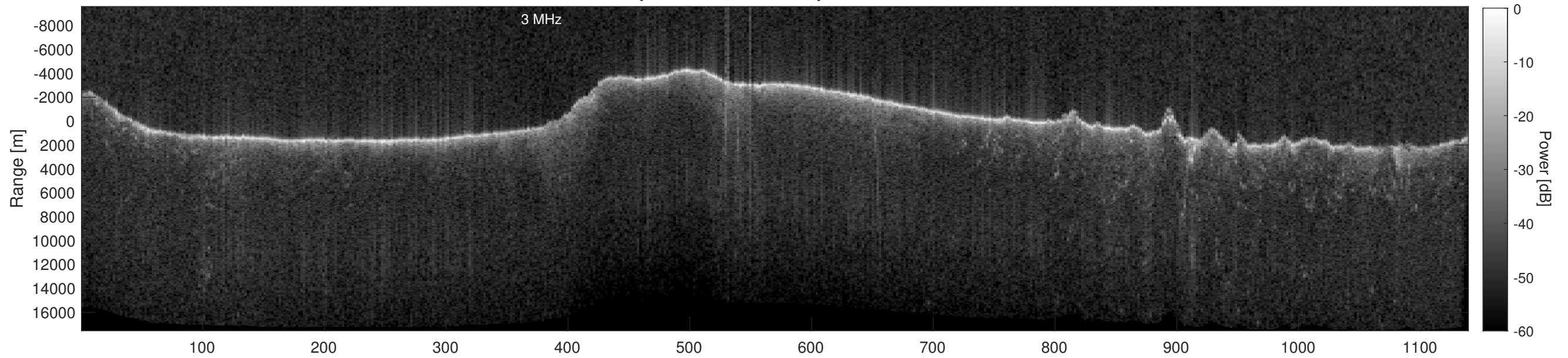
Orbit 13384, Depth-Corrected Cluttergram
