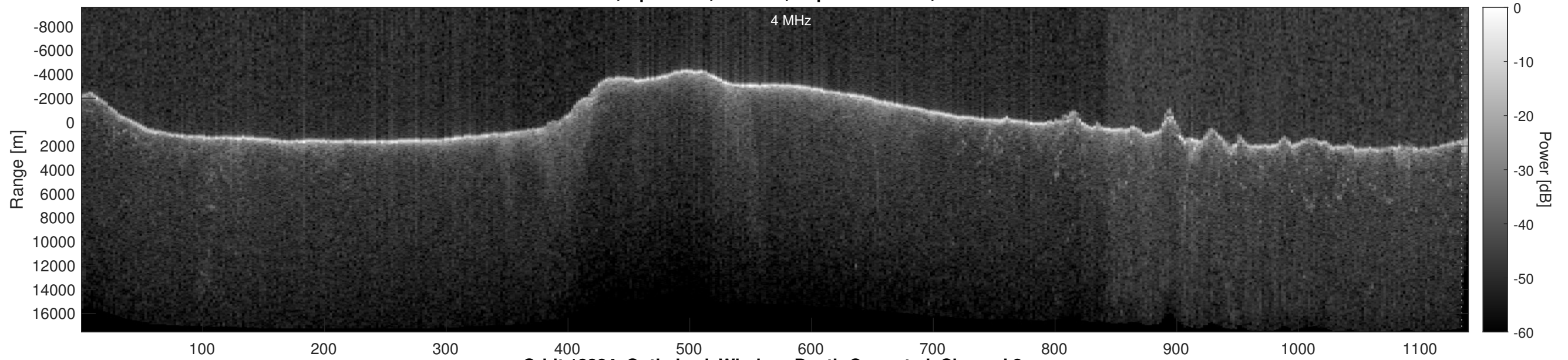
Orbit 13384, Optimized, Window, Depth-Corrected, Channel 2
