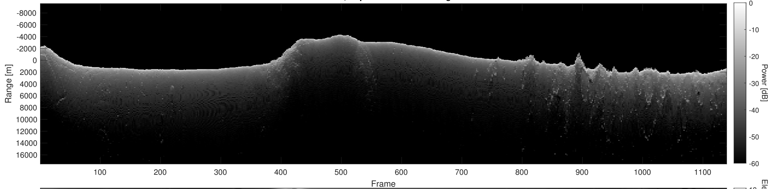
Orbit 13384, Depth-Corrected Cluttergram
