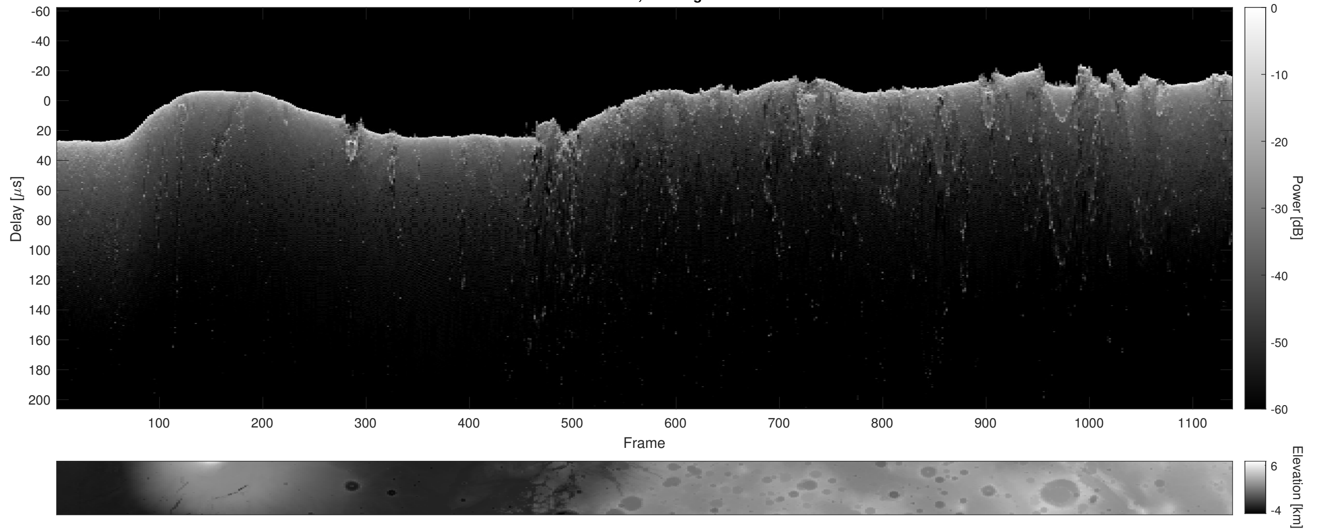
Orbit 13385, Cluttergram
