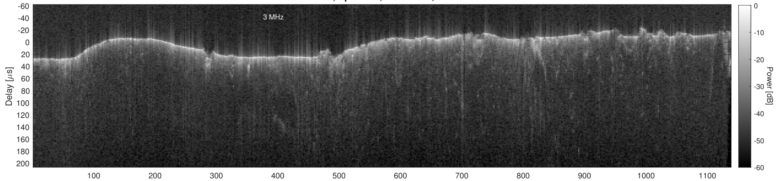
Orbit 13385, Cluttergram
