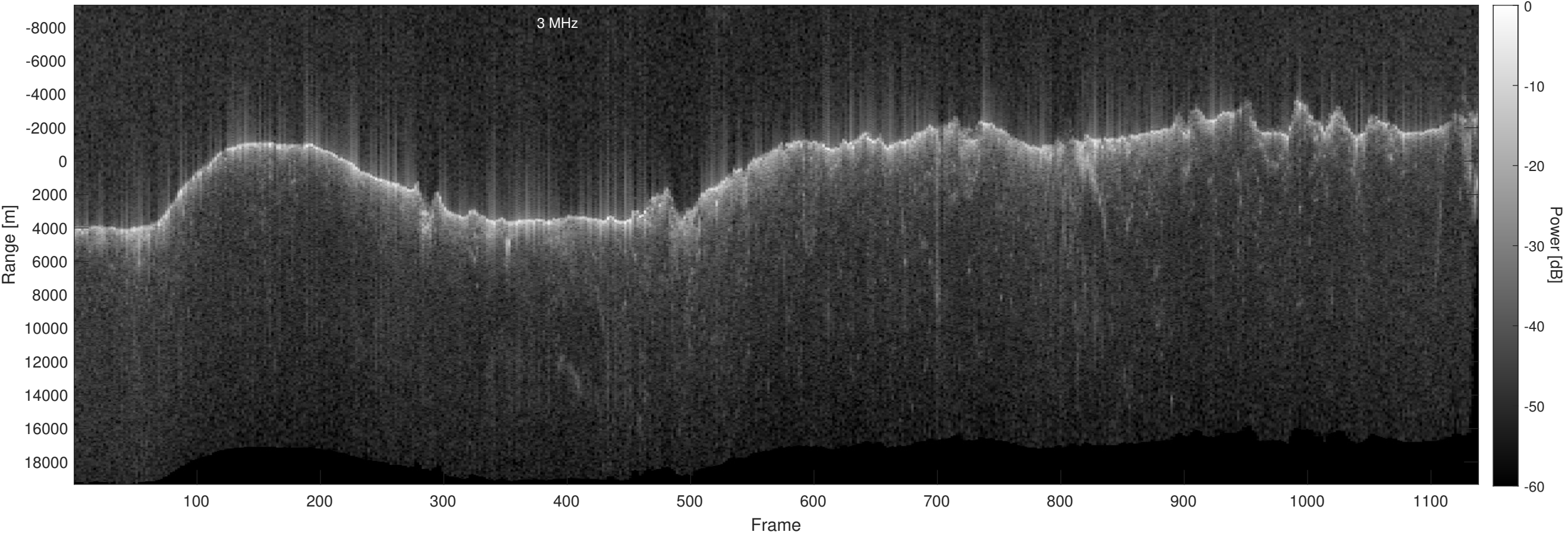
Orbit 13385, Optimized, No Window, Depth-Corrected, Channel 2
