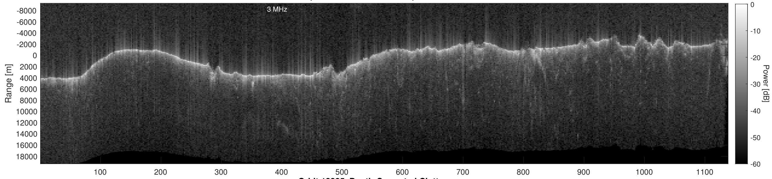
Orbit 13385, Depth-Corrected Cluttergram
