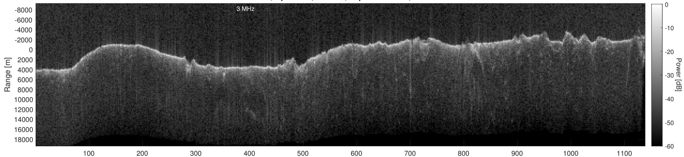
Orbit 13385, Depth-Corrected Cluttergram
