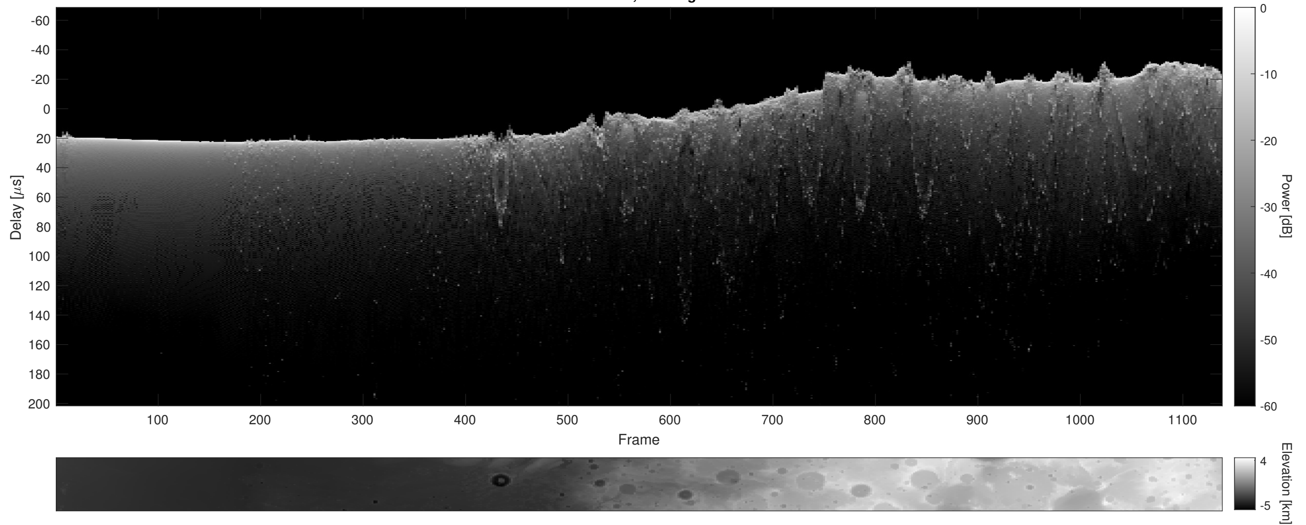
Orbit 13388, Cluttergram
