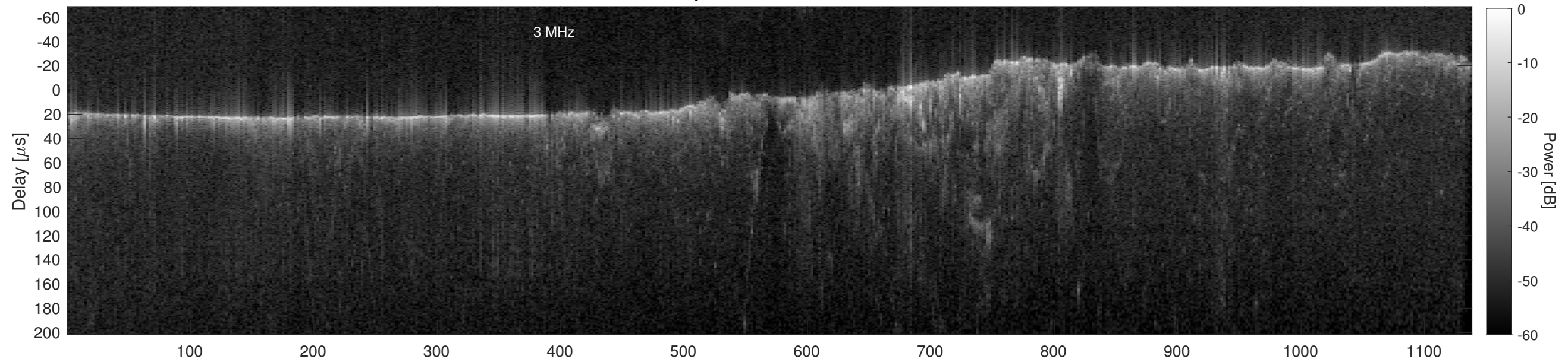
Orbit 13388, Cluttergram
