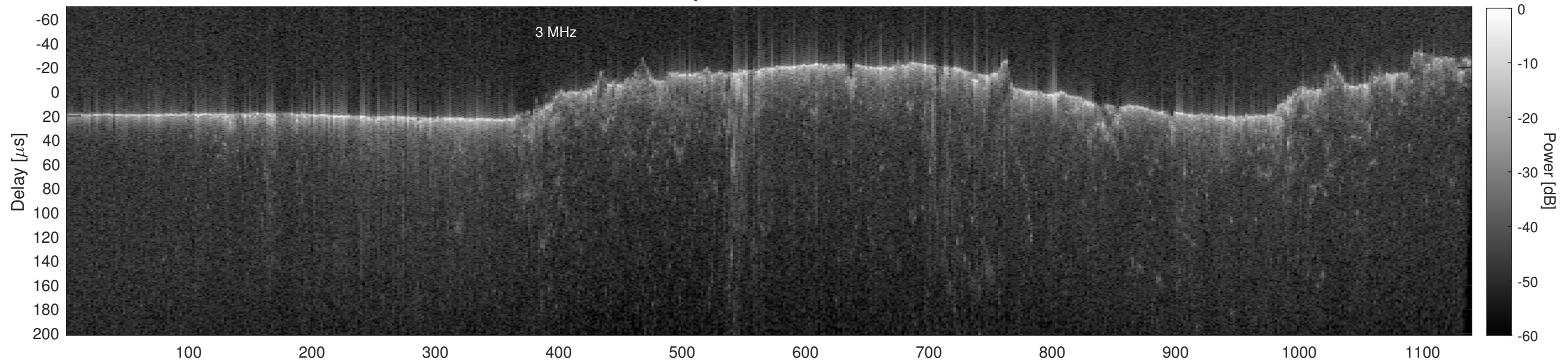
Orbit 13389, Cluttergram
