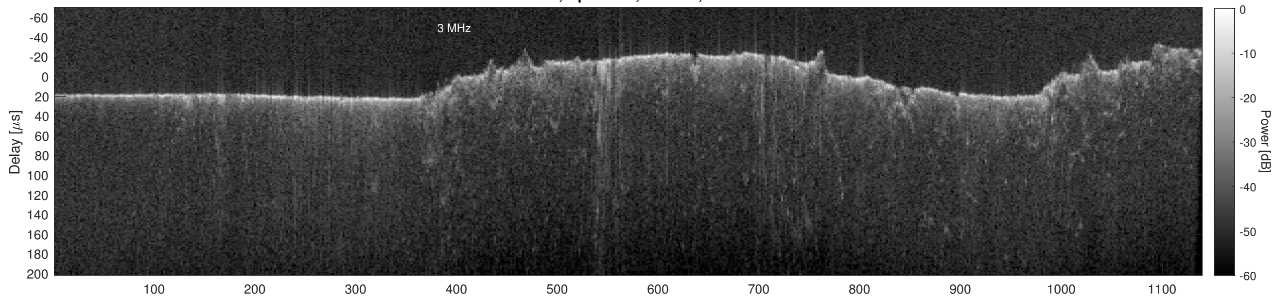
Orbit 13389, Cluttergram
