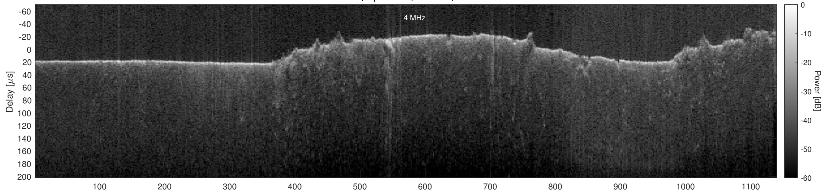
Orbit 13389, Optimized, Window, Channel 2
