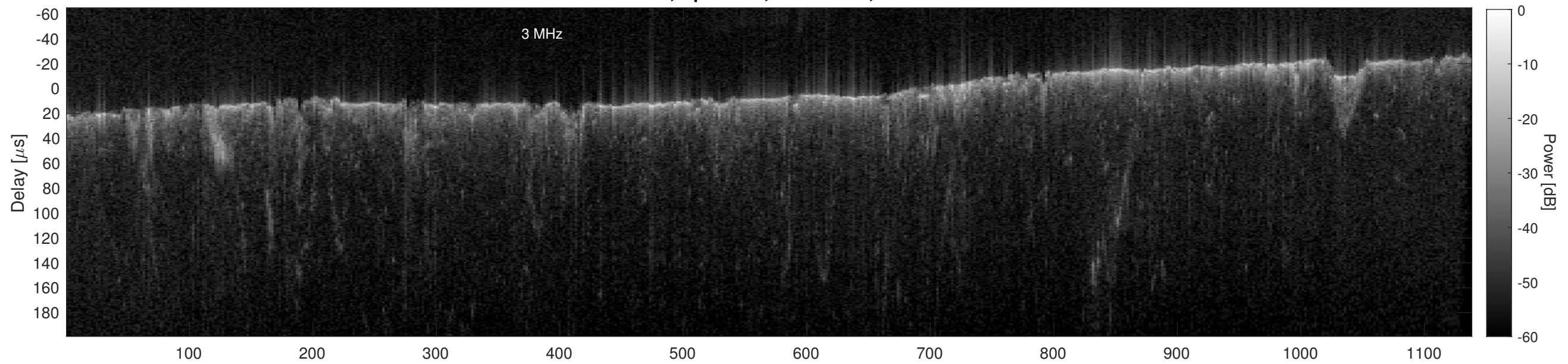
Orbit 13390, Cluttergram
