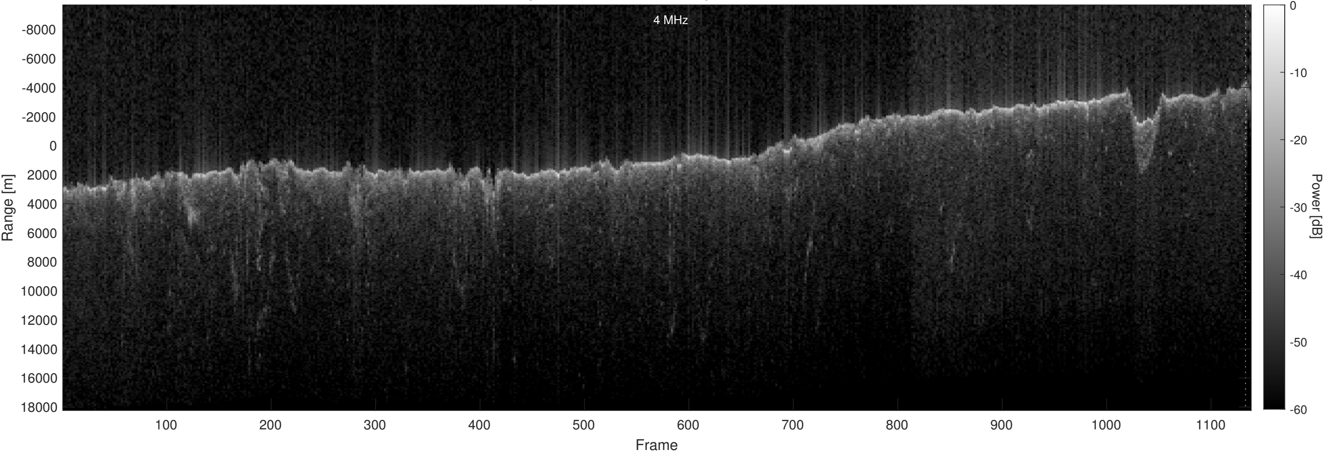
Orbit 13390, Optimized, No Window, Depth-Corrected, Channel 2
