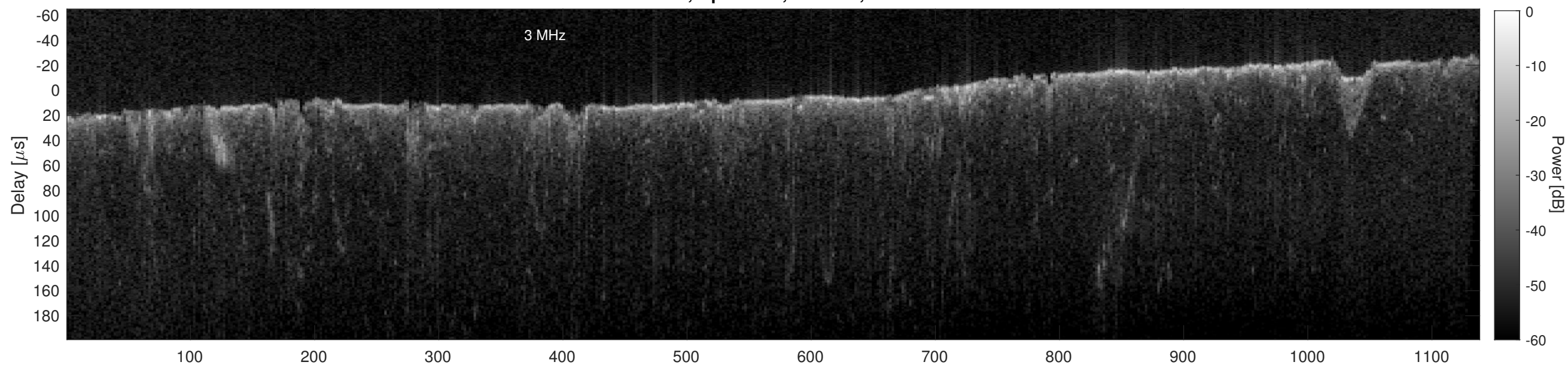
Orbit 13390, Cluttergram
