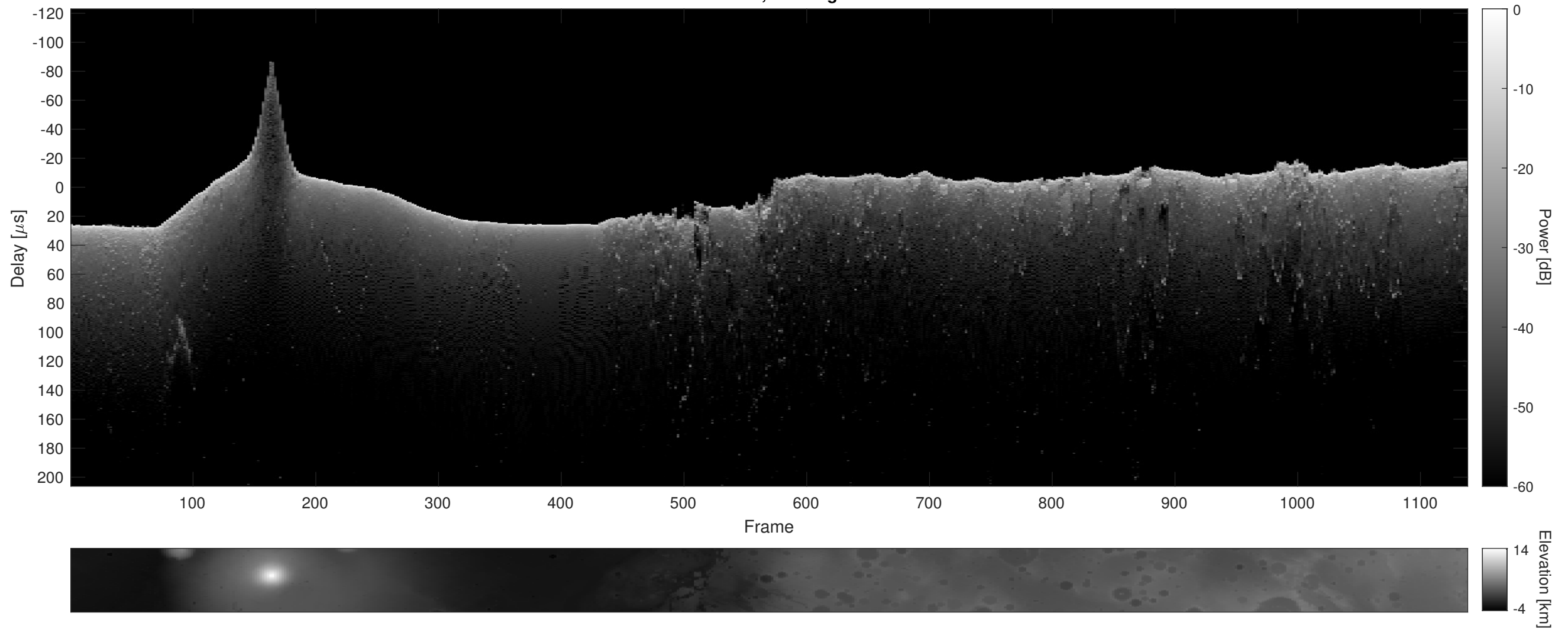
Orbit 13392, Cluttergram
