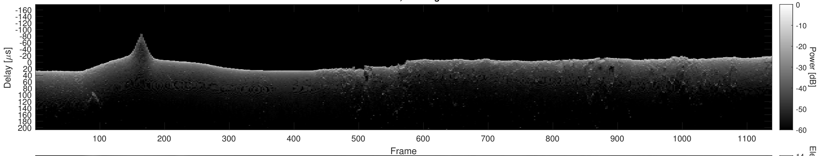
Orbit 13392, Cluttergram
