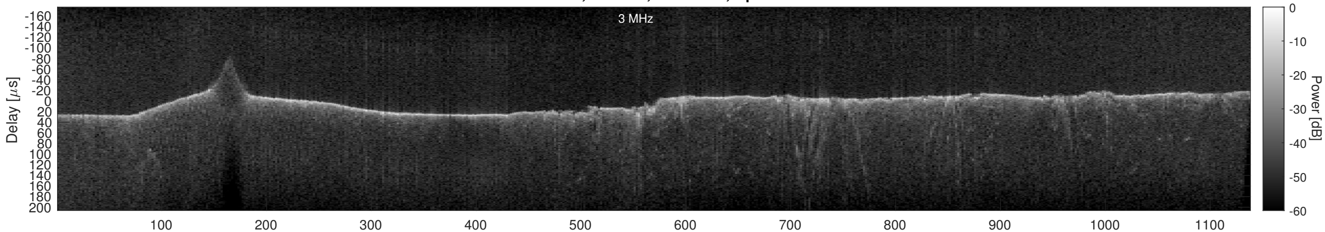
Orbit 13392, Cluttergram
