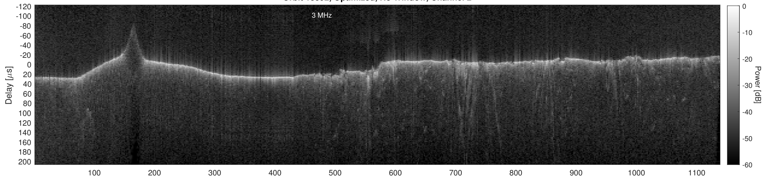
Orbit 13392, Cluttergram
