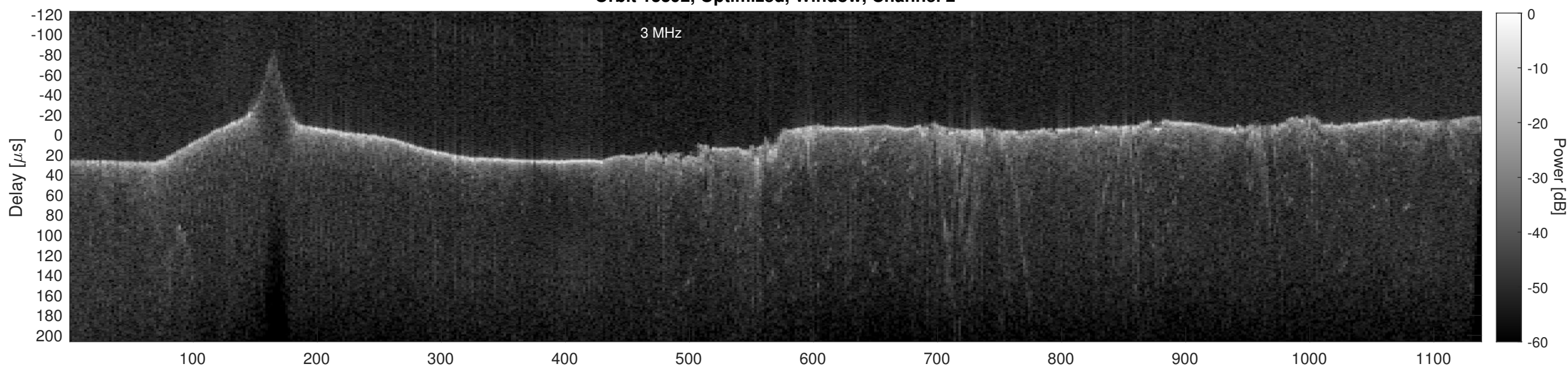
Orbit 13392, Cluttergram
