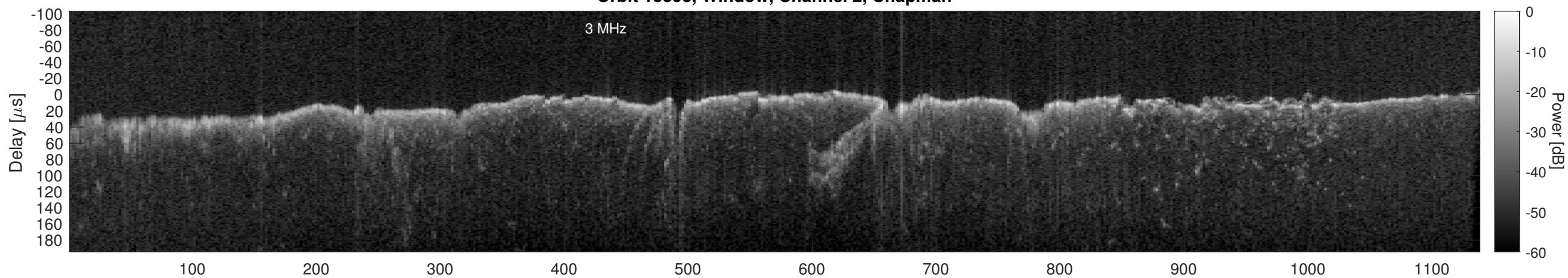
Orbit 13393, Window, Channel 2, Optimized
