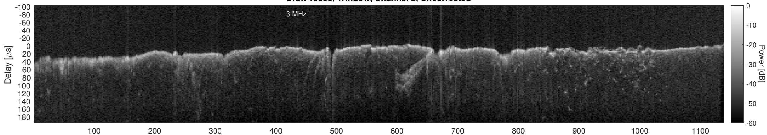
Orbit 13393, Window, Channel 2, Chapman
