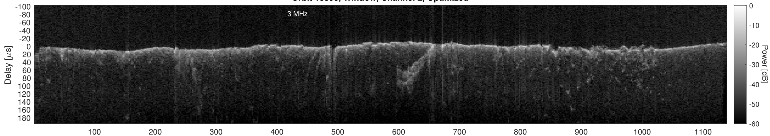
Orbit 13393, Cluttergram
