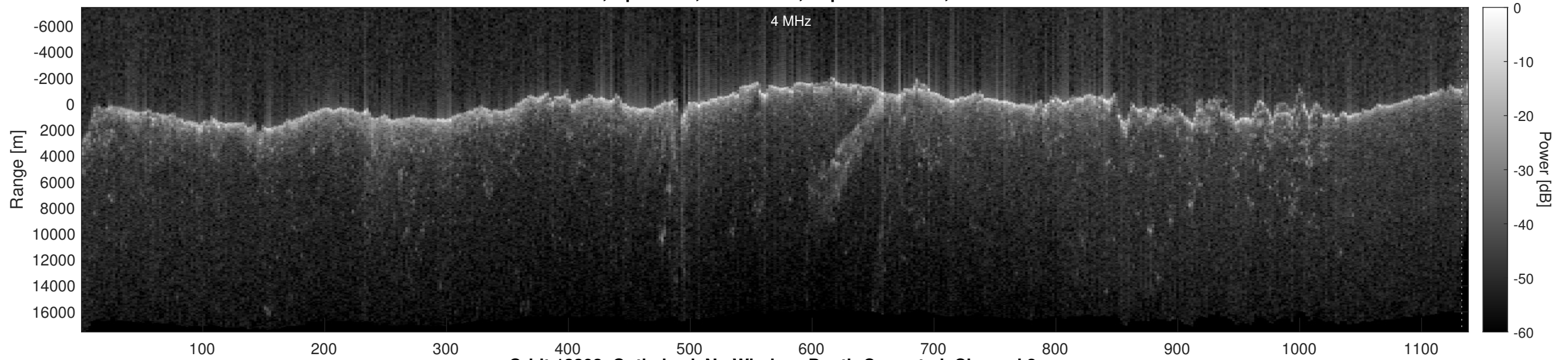
Orbit 13393, Optimized, No Window, Depth-Corrected, Channel 2
