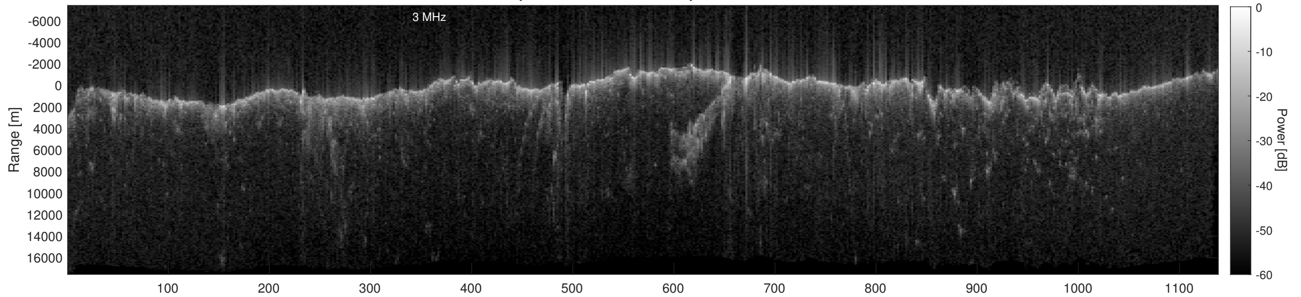
Orbit 13393, Depth-Corrected Cluttergram
