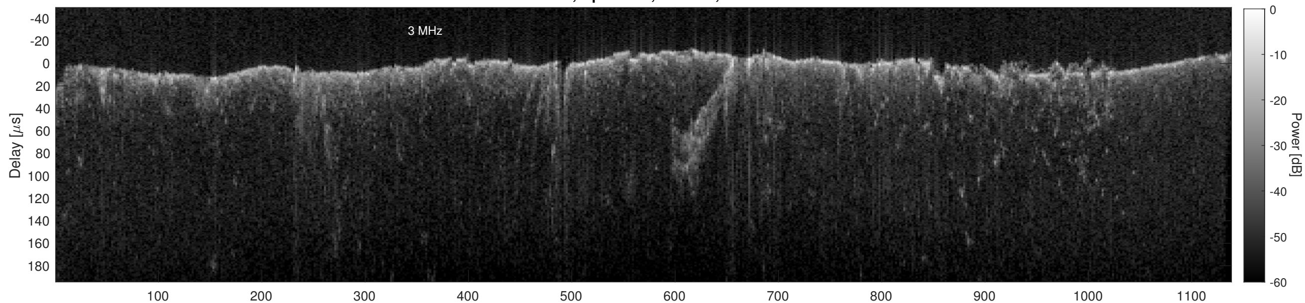
Orbit 13393, Cluttergram
