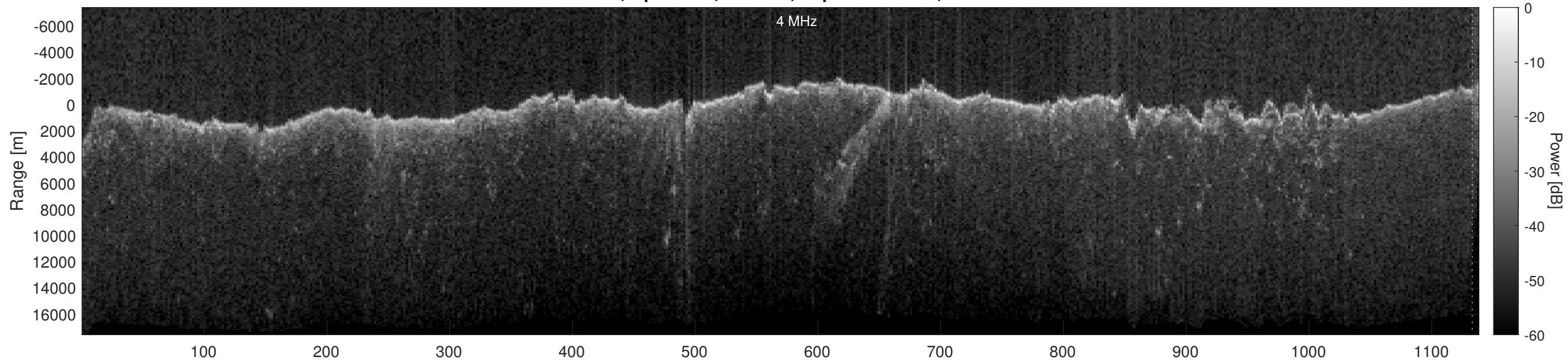
Orbit 13393, Optimized, Window, Depth-Corrected, Channel 2
