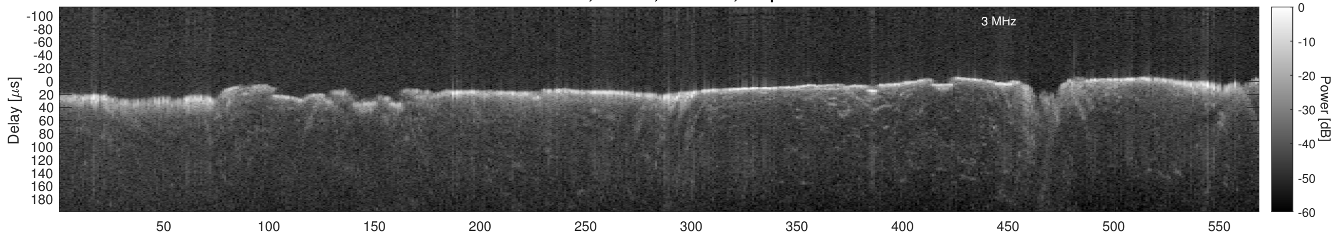
Orbit 13394, Window, Channel 2, Optimized
