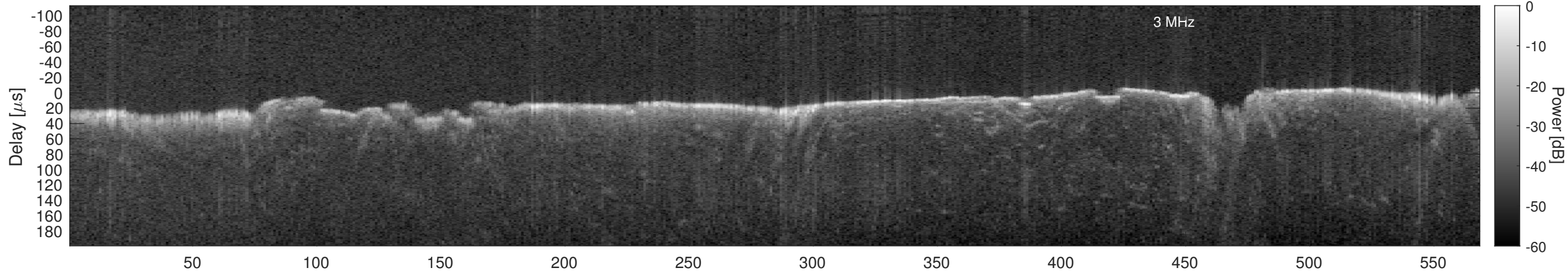
Orbit 13394, Window, Channel 2, Chapman
