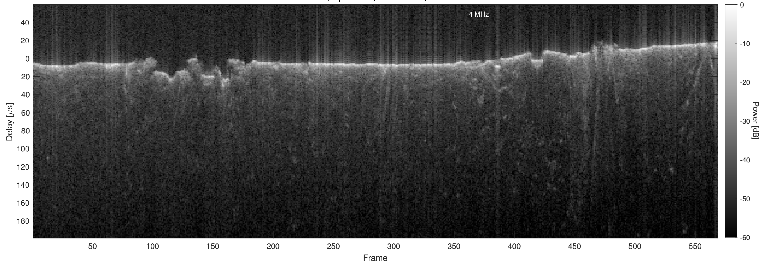
Orbit 13394, Optimized, No Window, Channel 2
