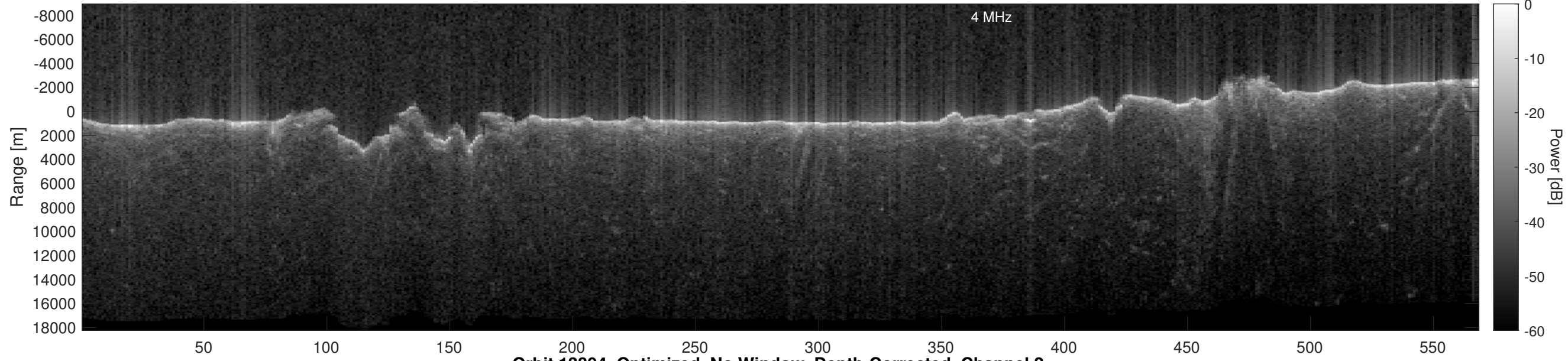
Orbit 13394, Optimized, No Window, Depth-Corrected, Channel 2
