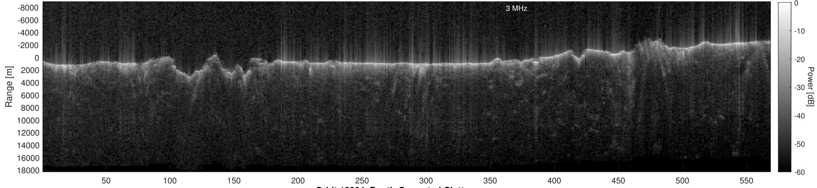
Orbit 13394, Depth-Corrected Cluttergram
