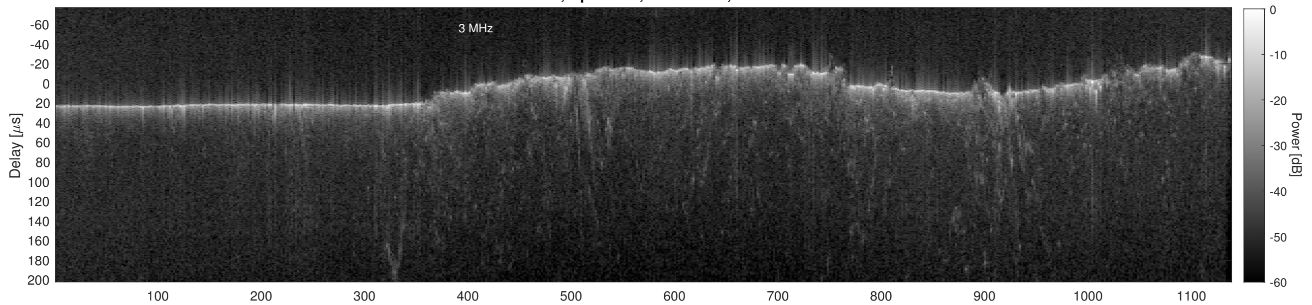
Orbit 13396, Cluttergram
