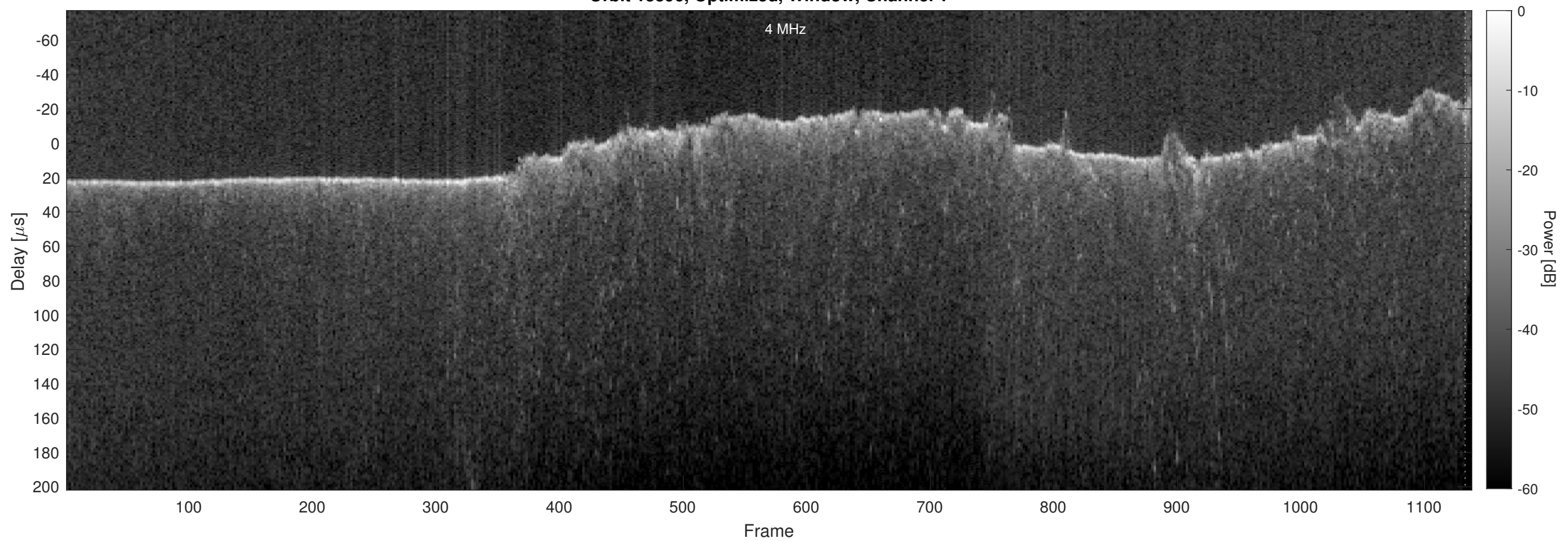
Orbit 13396, Optimized, Window, Channel 2
