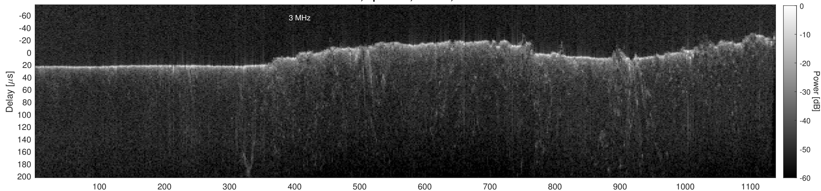
Orbit 13396, Cluttergram
