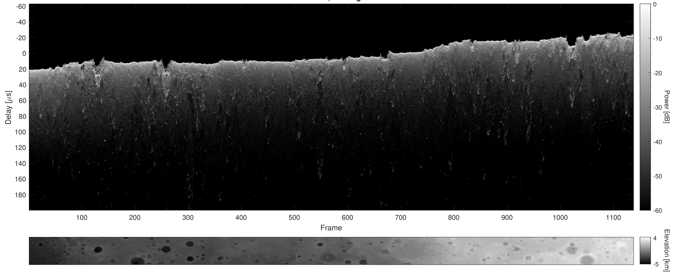
Orbit 13397, Cluttergram
