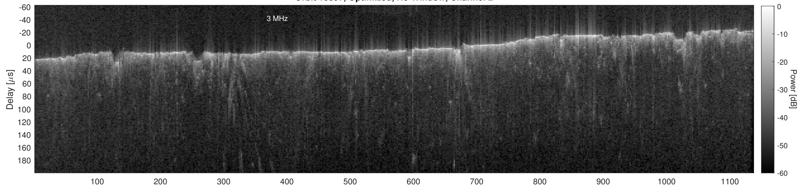
Orbit 13397, Cluttergram
