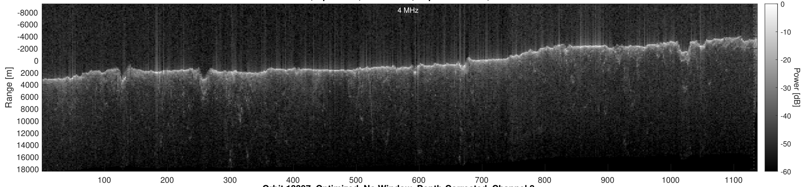
Orbit 13397, Optimized, No Window, Depth-Corrected, Channel 2
