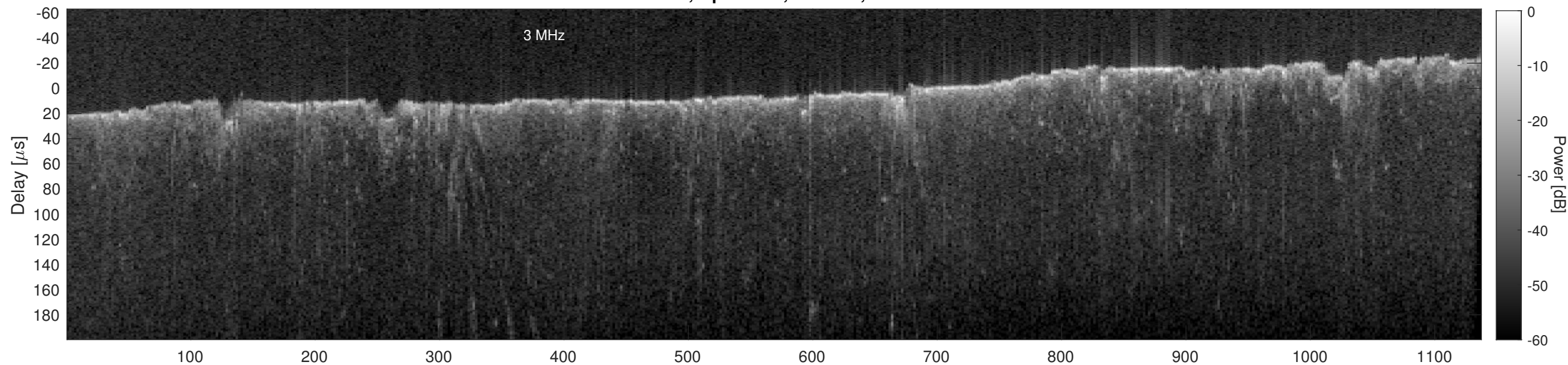
Orbit 13397, Cluttergram
