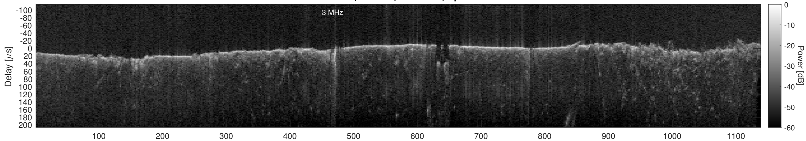
Orbit 13401, Cluttergram
