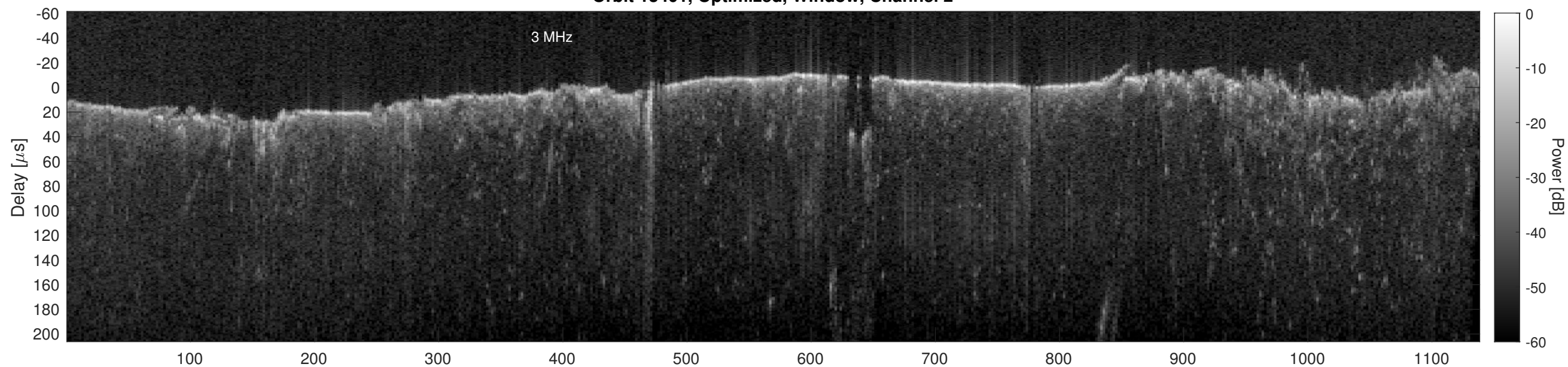
Orbit 13401, Cluttergram
