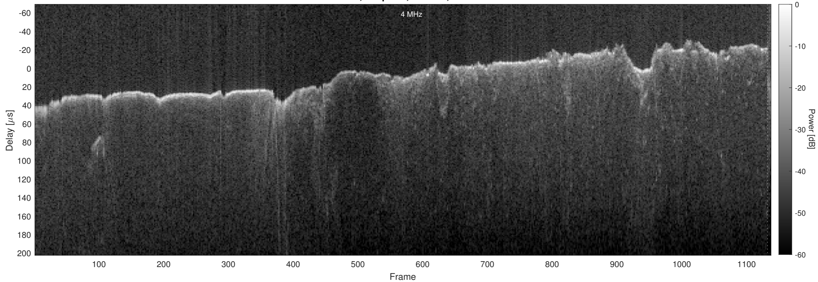
Orbit 13402, Chapman, Window, Channel 2
