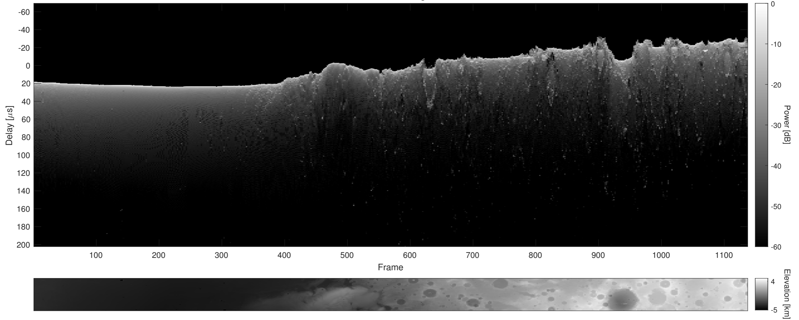
Orbit 13402, Cluttergram
