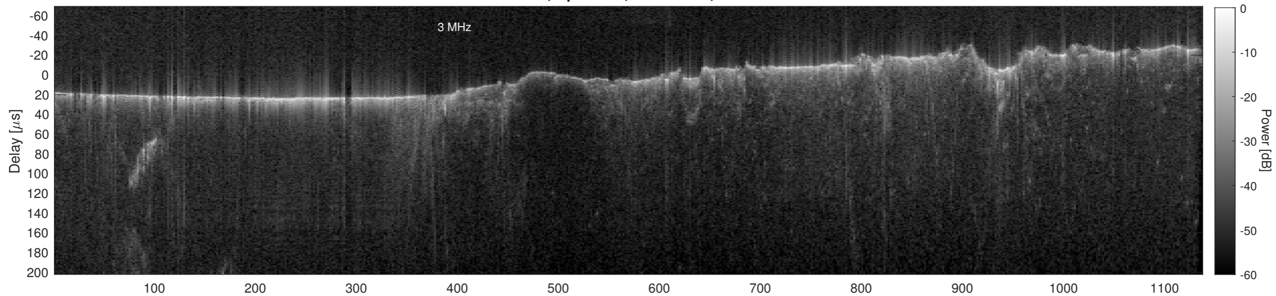
Orbit 13402, Cluttergram
