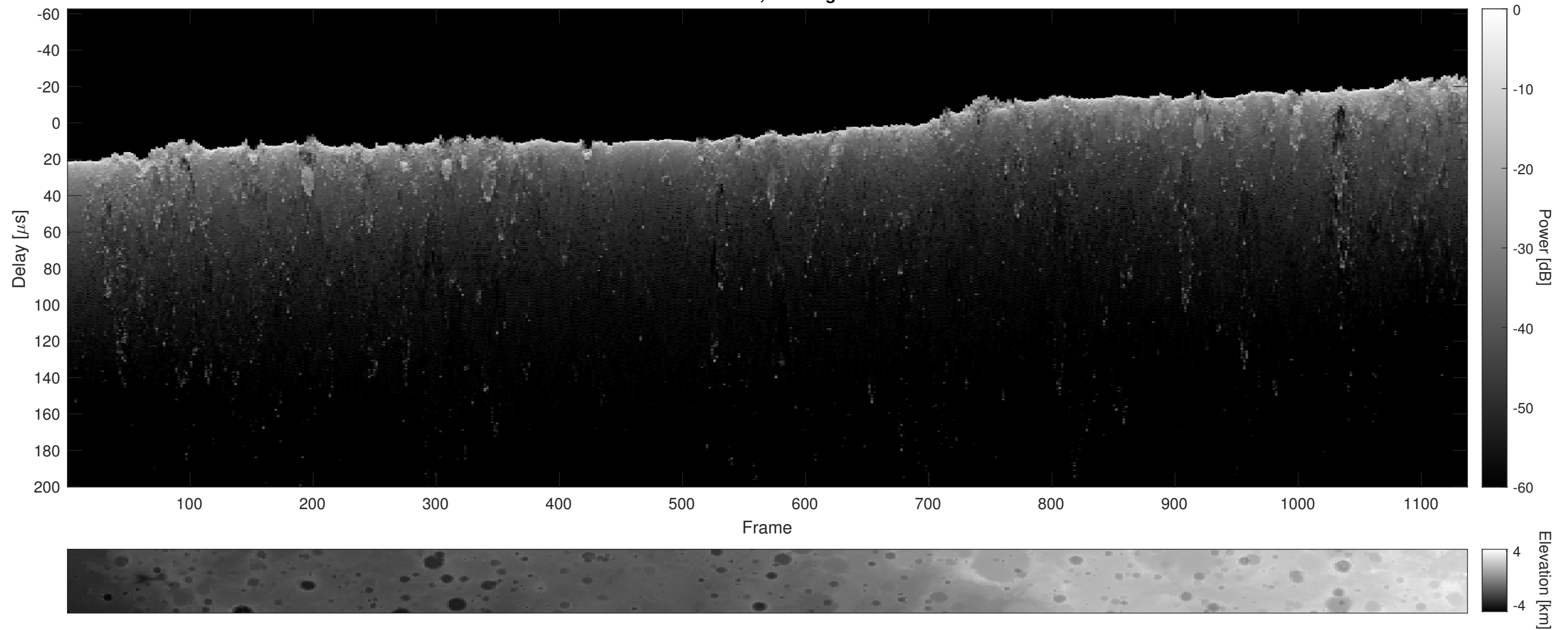
Orbit 13404, Cluttergram
