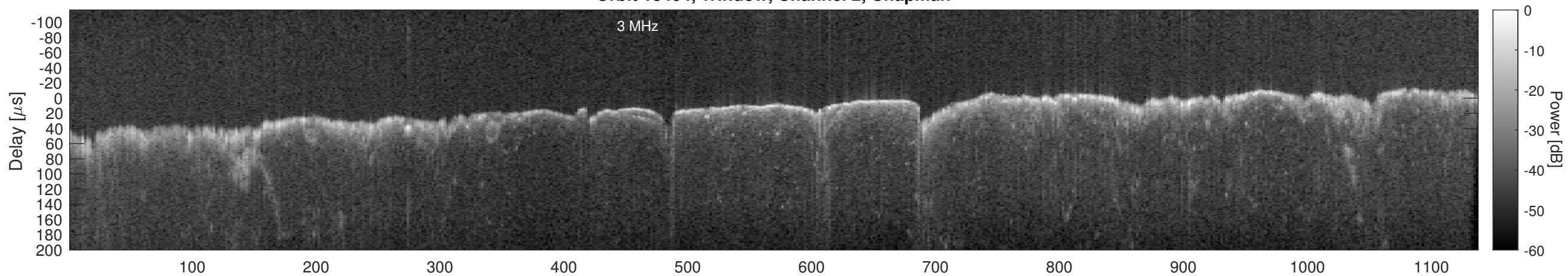
Orbit 13404, Window, Channel 2, Optimized
