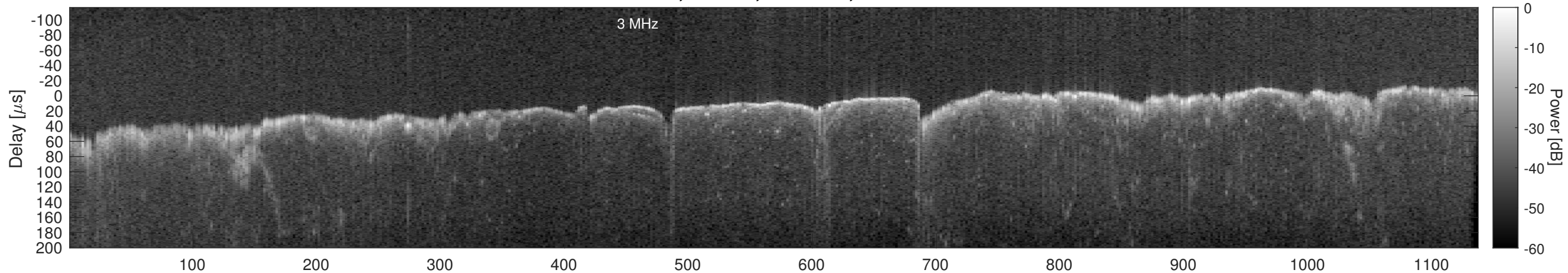
Orbit 13404, Window, Channel 2, Chapman
